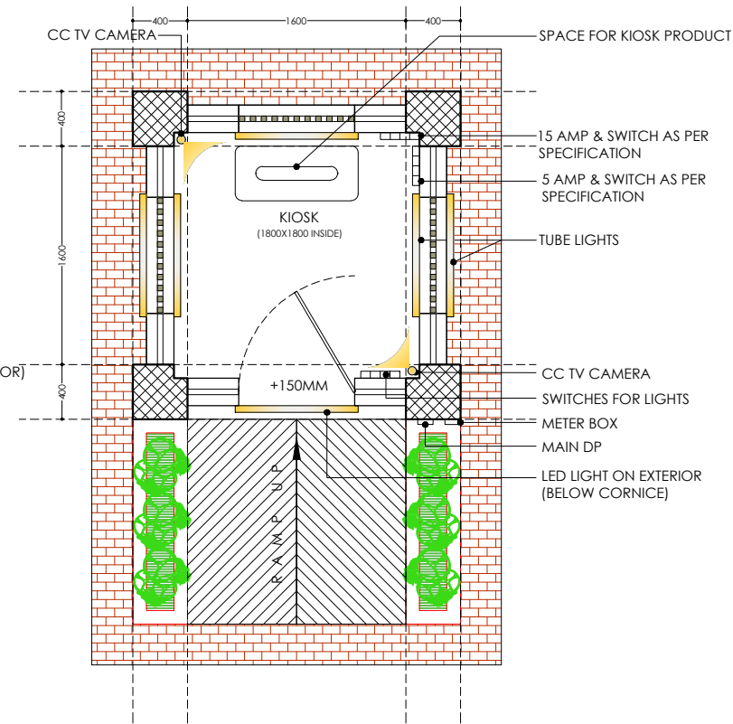
DRAWING 2 ELECTRICAL FIXTURE
