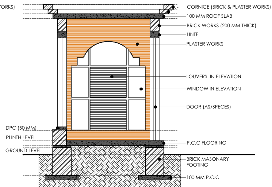
DRAWING 6 SECTION 2 - THRU S2
