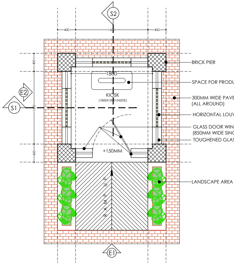
DRAWING 1 FLOOR PLAN
