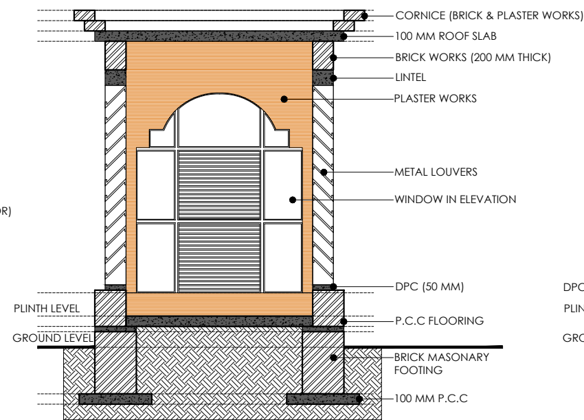
DRAWING 5 SECTION 1 - THRU S1
